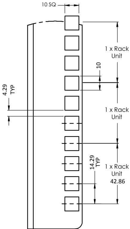
ESU PROFILE Equally Spaced Unit
